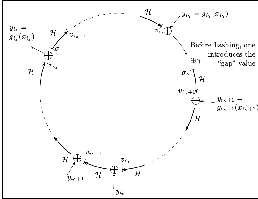
Fig. 2. The modified ring. The signer starts from index i_s and value \sigma and he closes the ring when computing v_{i_s} , using his trapdoor. The verifier starts from i_0 with value v_{i_0} and checks whether the last hash outputs v_{i_0} . A “simulator” starts from i_\gamma and a seed \sigma_\gamma to define \gamma at closure only, when computing v_{i_\gamma} . \mathcal{H} is a public hash function.
