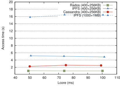
(a) – Mean writing time (second) as a function of the L_{Core} latency
