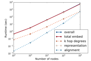
Figure 7: REGAL is sub-quadratic.
